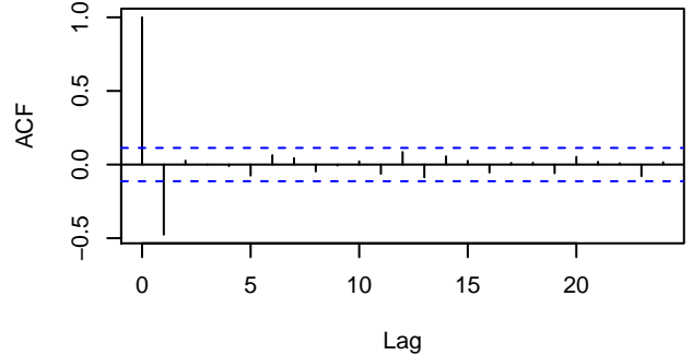
Series diff(y1)
