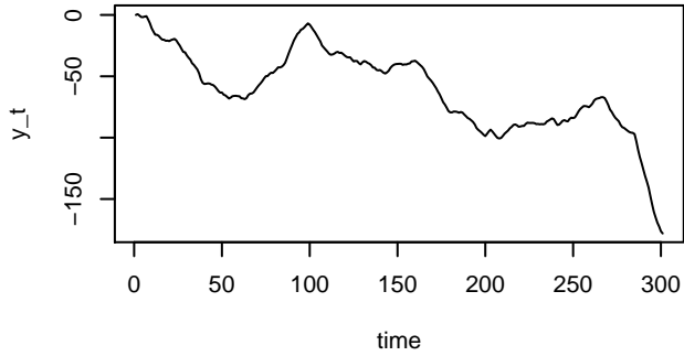
Series y_3
