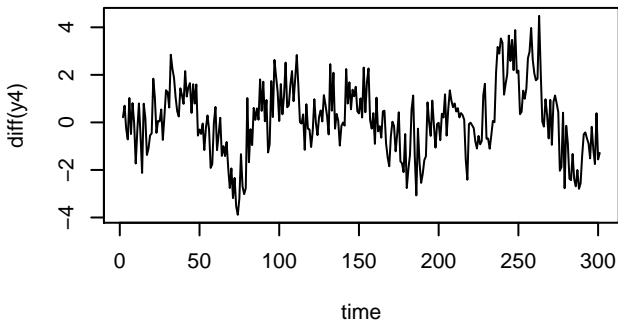
Series diff(y4)
