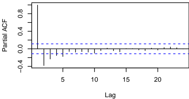
Series y4
