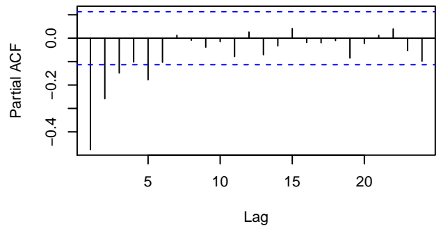
Series diff(y1)
