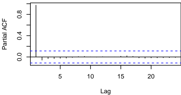
Series y_3
