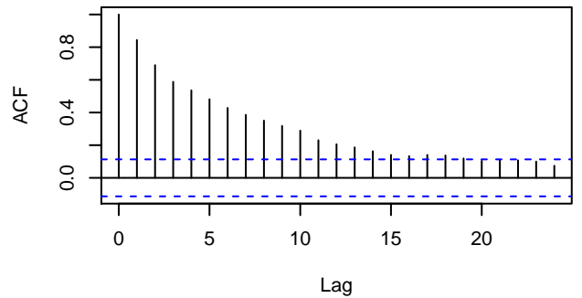
Series \text{diff}(y_3)
