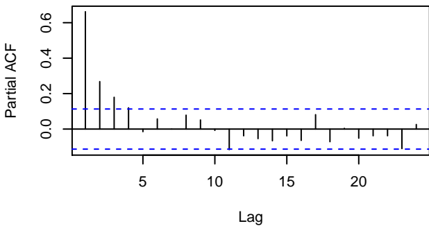
Series diff(y4)
