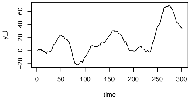
Series y4
