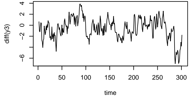
Series \text{diff}(y_3)
