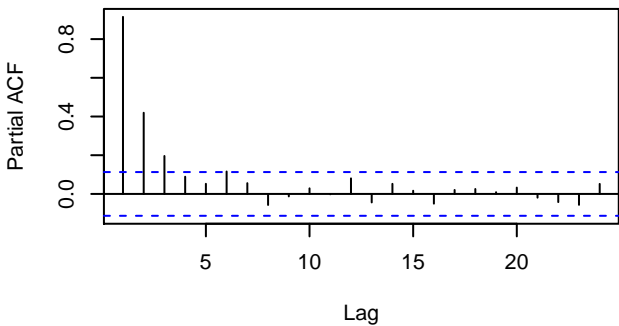
Series y1
