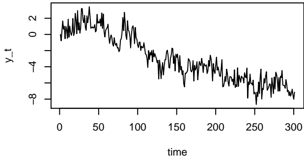
Series y1
